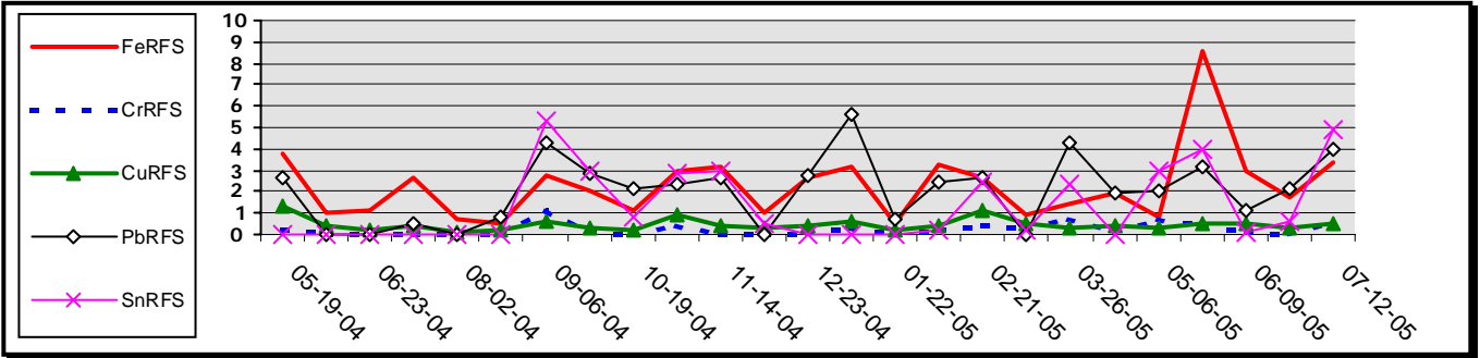
Wear Metals by RDE
